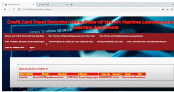
Fig.4. User details.
