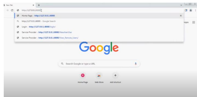
Fig.1. Home page.
