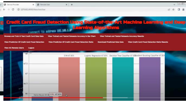
Fig.8. Prediction Graphs.
