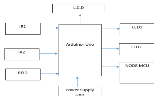
Fig1: Proposed block diagram ARDUINO-UNO:
