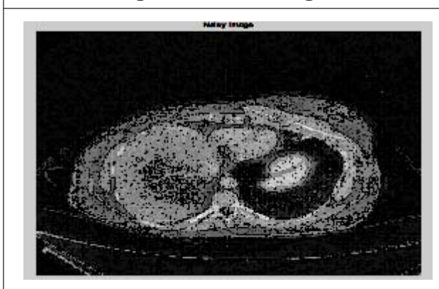
Figure 4: Noise Image
