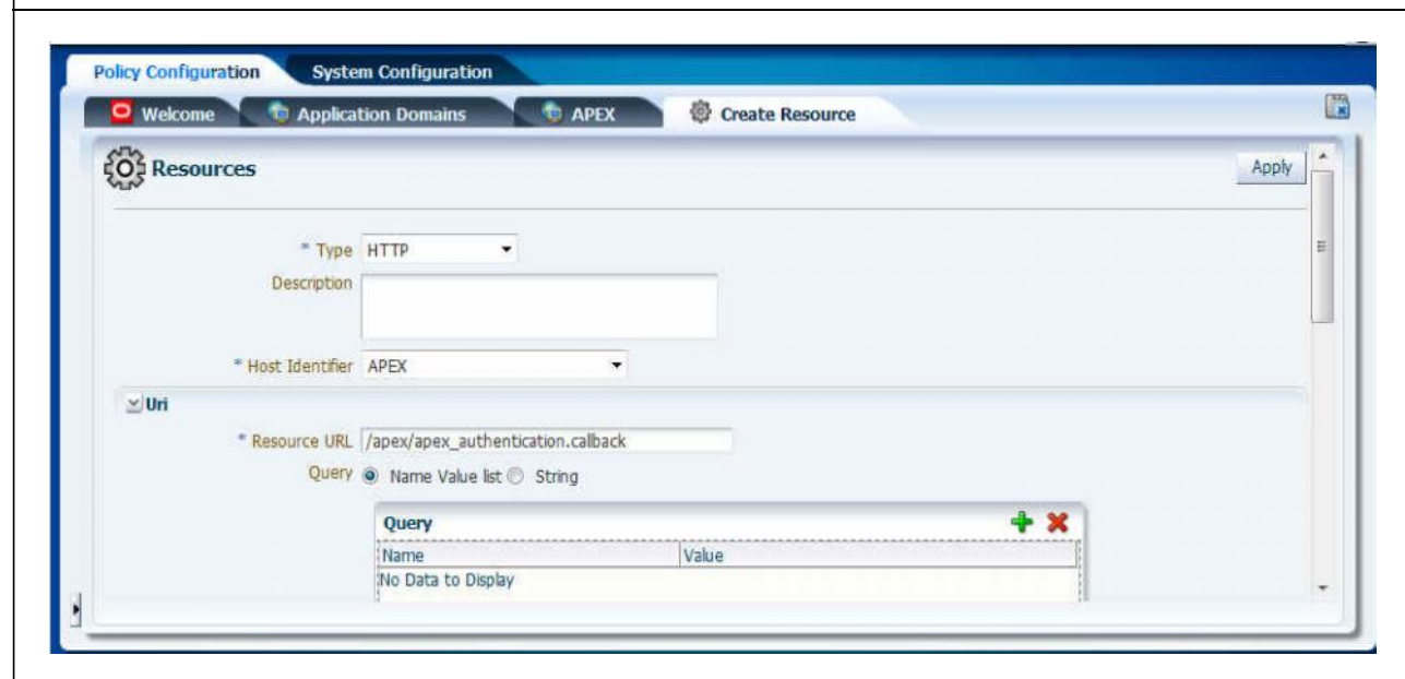
Figure 10: Policy Configuration
