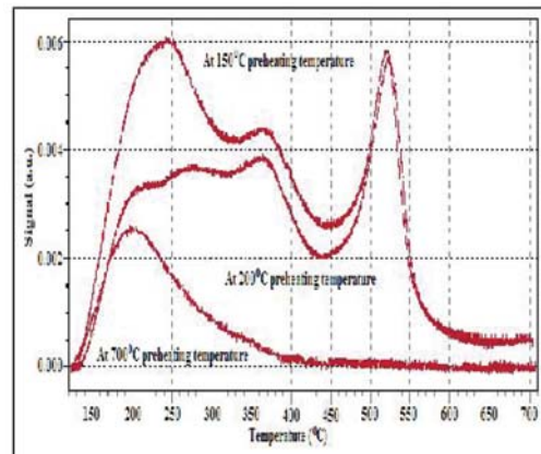
Figure 18: NH 3 -TPD patterns of 12-TPA/ZrO 2 -20 at different preheating temperatures
